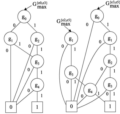
Fig. 7. ZBDDs for vertical seeds.
