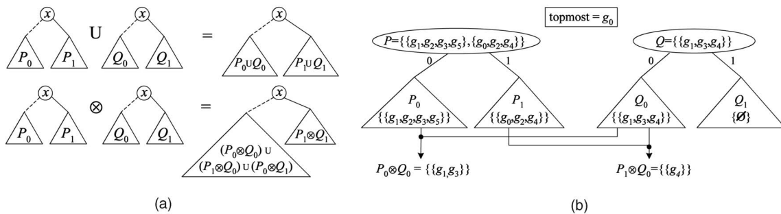
Fig. 15. The operators \cup and \otimes on ZBDDs. (a) The set operators are recursively defined on the ZBDDs. The operator \cap is defined in the same way as the operator \otimes , but is not shown here. (b) An example.
