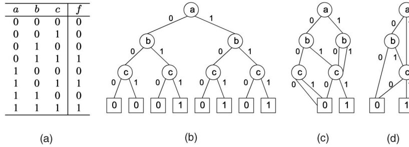
Fig. 3. Representations of a Boolean logic function f = (a + b)c . (a) Truth table. (b) BDD for the variable order (a, b, c) . (c) After applying the first reduction rule. (d) After applying the second reduction rule. This corresponds to the ROBDD for the variable order (a, b, c) .
